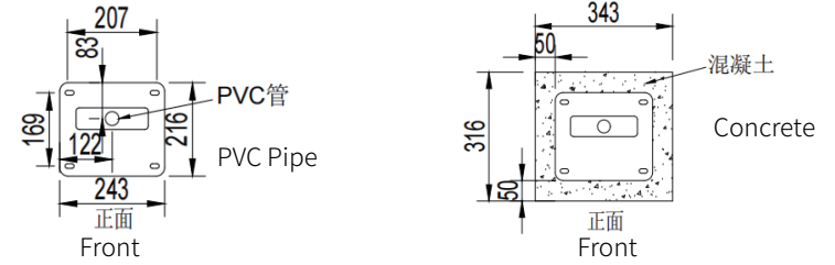
Schematic diagram of foundation opening
